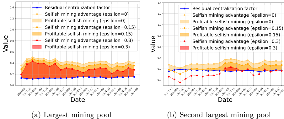
Fig. 2: Periods of profitable selfish mining. According to Thm. 1, selfish mining becomes more profitable than honest mining when the selfish mining advantage of a mining pool (defined as the right-hand side of inequality (5)) surpasses its residual centralization factor (defined in Def. 10).
