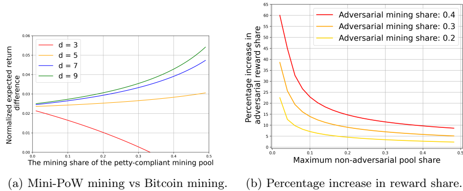
Fig. 7: Quantitative analysis of the distraction attack.
